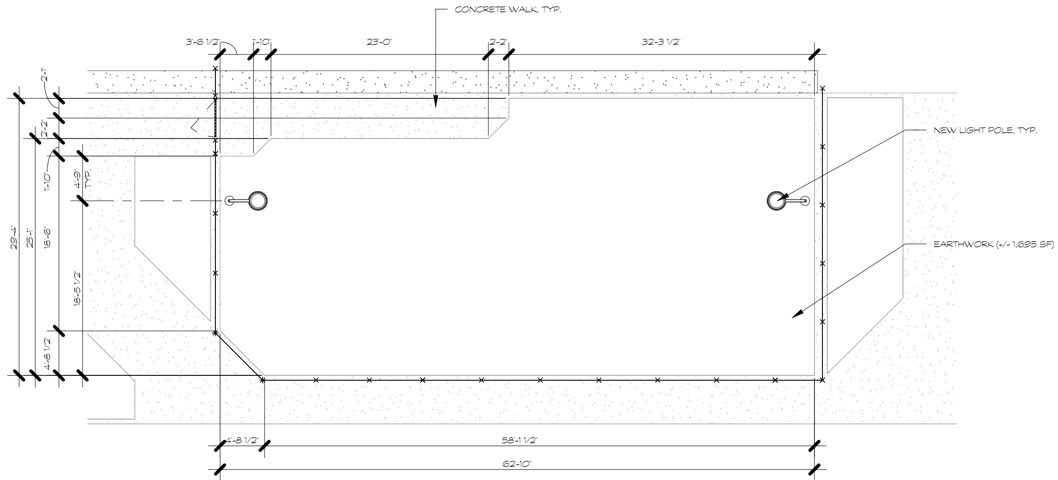
① SOUTH PLAY STRUCTURE 1" = 10'-0"
