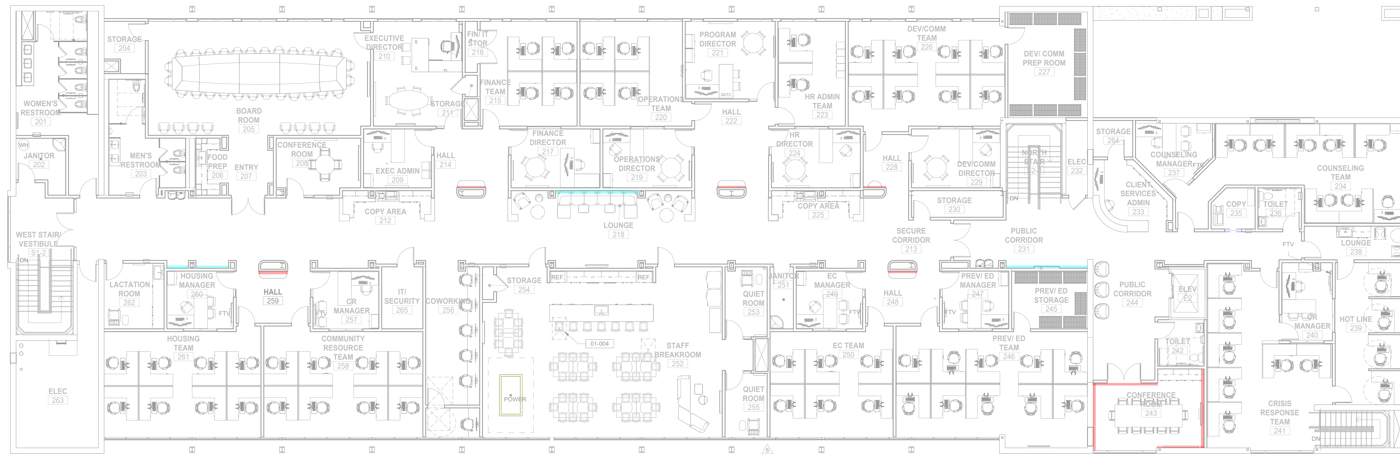
SECOND FLOOR FURNITURE + POWER + DATA PLAN
